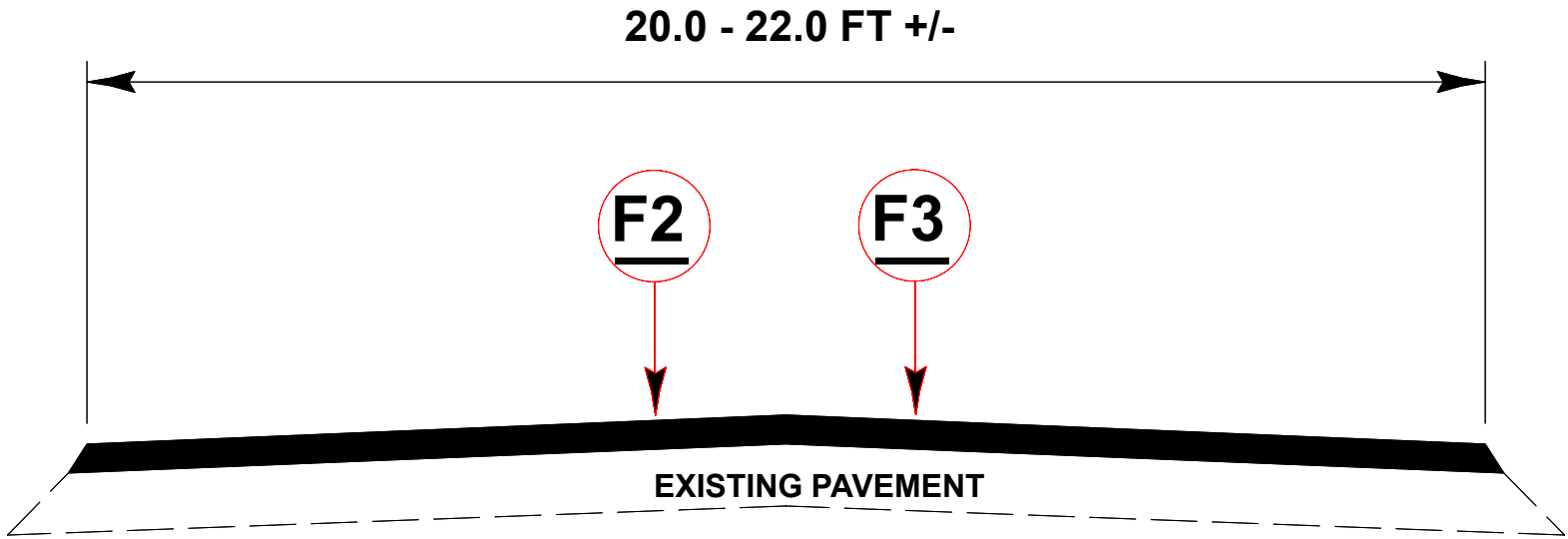
TYPICAL SECTION # 2 MAP(S) # 2 & 3
